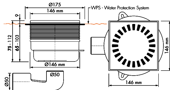
horizontal outlet
